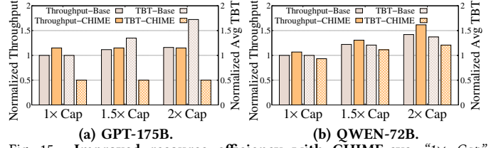
Fig. 15. Improved resource efficiency with CHIME-sys. “1x Cap” denotes the basic memory capacity (2TB for GPT-175B and 1TB for QWEN-72B) according to Table II. The results are evaluated using the OpenR1 trace.
