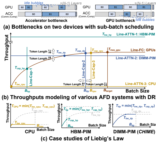
Fig. 2. CHIME's Disaggregated Roofline Model and case studies. "DIMM-PIM" denotes CHIME's proposal, leveraging DIMM-based host memory with bank-level PUs as the accelerator. "Throughput" denotes tokens per second.
