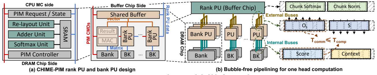
Fig. 7. CHIME-PIM design with bubble-free pipelining.
