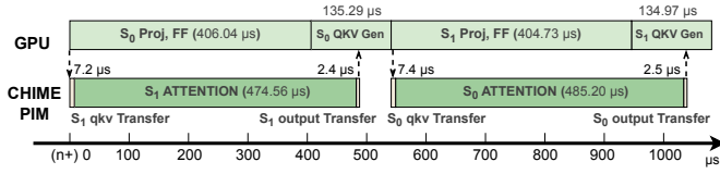
Fig. 17. Decode execution timeline of CHIME pipeline for single LLM layer. The batch is executed with GPT-175B and the OpenR1 trace.
